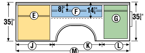
"A" Compartment Layout
