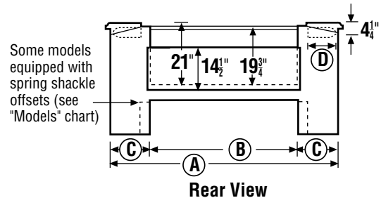
"B" Compartment Layout
