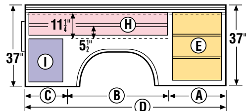
"B" Compartment Layout
