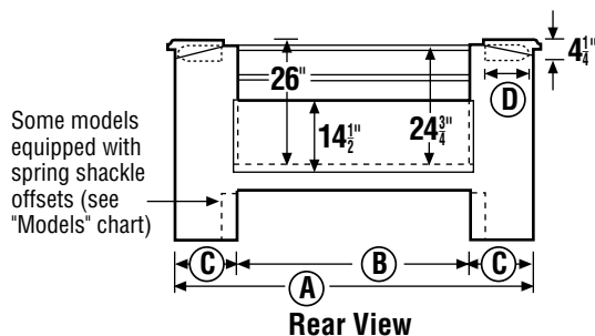
"B" Compartment Layout
