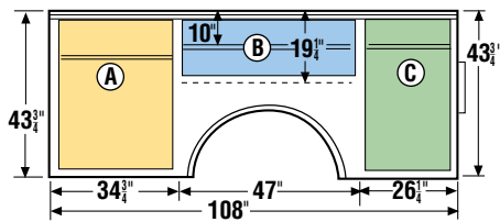
HD108AB "A" Compartment Layout
