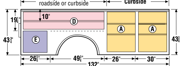
"B" Compartment Layout
