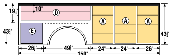
"B" Compartment Layout
