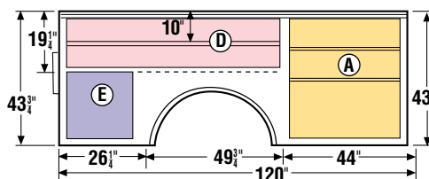
"B" Compartment Layout
