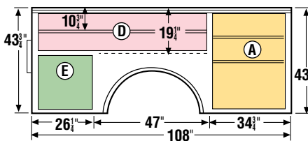
"B" Compartment Layout
