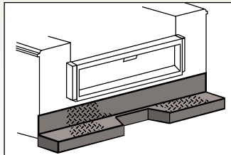
Deck plate step bumper with recess
