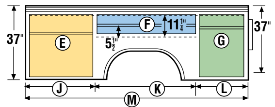
"A" Compartment Layout
