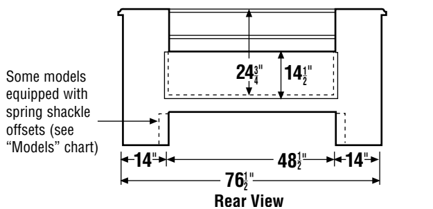
"B" Compartment Layout
