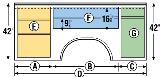
"A" Compartment Layout
